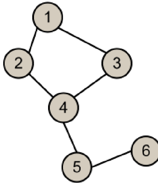
Undirected Graph
