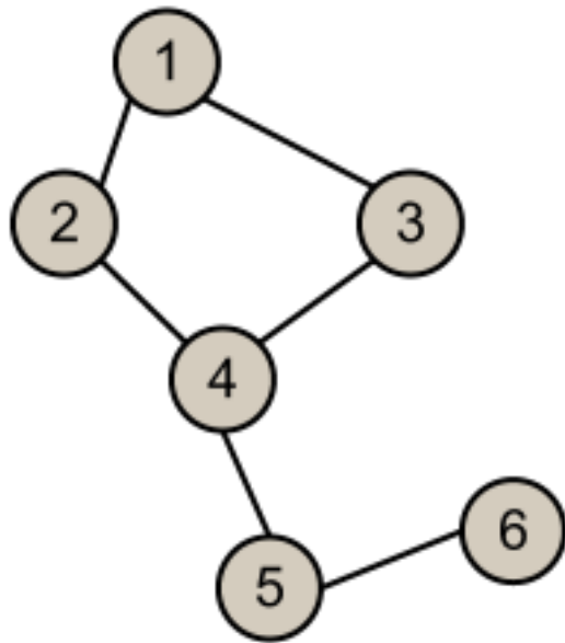
Undirected Graph
